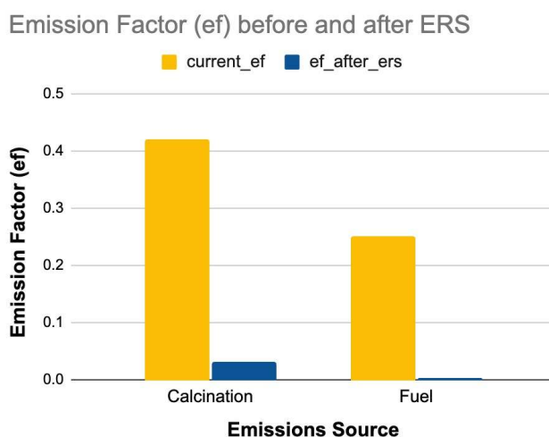
Figure 7 Average direct emission factors (tCO 2 per tonne of cement) from calcination and fuel combustion before (yellow bars) and after (blue bars) the application of emission reduction strategies (ERS) across cement assets worldwide.
