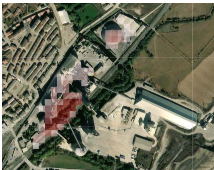
Figure 6 Satellite-detected hotspots over Valderrivas cement plant in Cantabria, Spain during August 2024.
