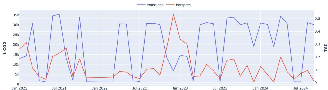
Figure 5 Satellite-based Thermal Anomaly Index (TAI; red solid line) and estimated emissions (blue solid line) at Valderrivas cement plant in Cantabria, Spain during January 2021 - September 2024.
