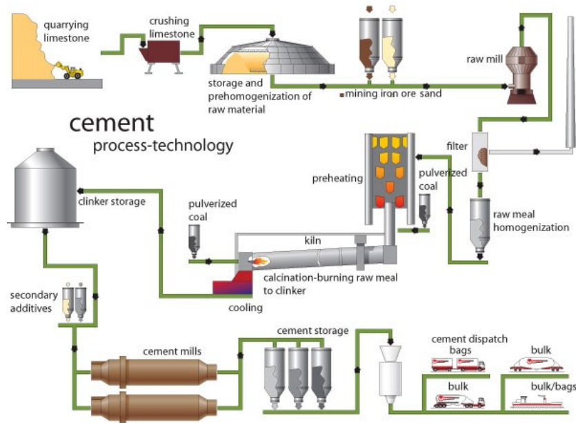
Figure 7 Overview of the cement production process (Construction Cost, 2016).
