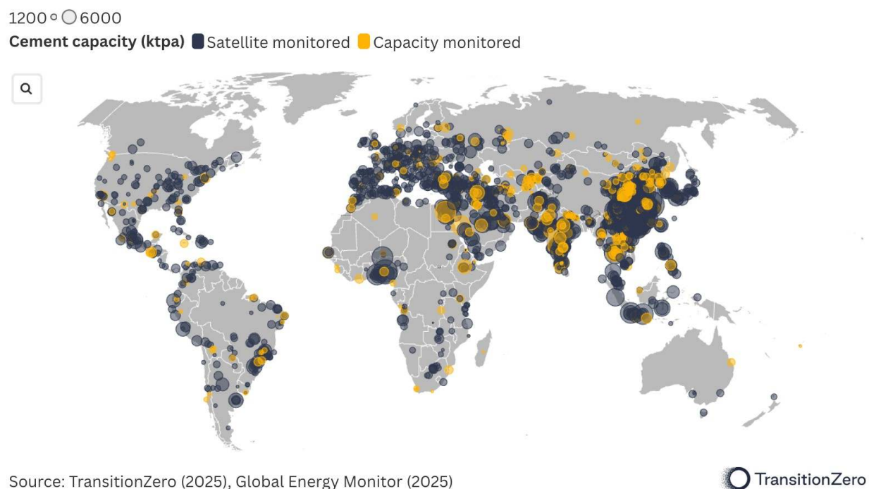
Figure 2 Global map showing integrated cement facilities. Countries included in cement emissions monitoring are shaded. Assets that are monitored with satellites are shown in blue. The circle size represents plant production capacity, with reference scales shown at the top of the figure for 1,200 and 6,000 thousand tonnes per annum (ktpa).
